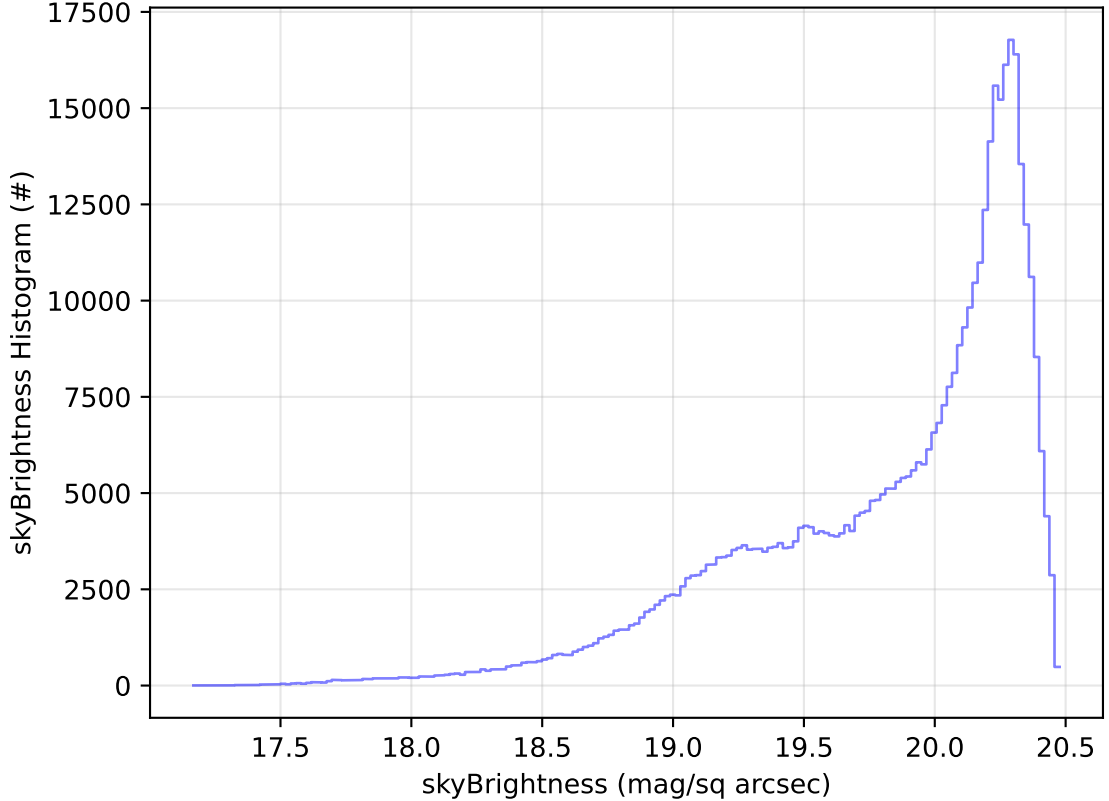
roll_uniform_eh_acc0.2_mjdp0_v3.4_10yrs All sky i band: skyBrightness Histogram
