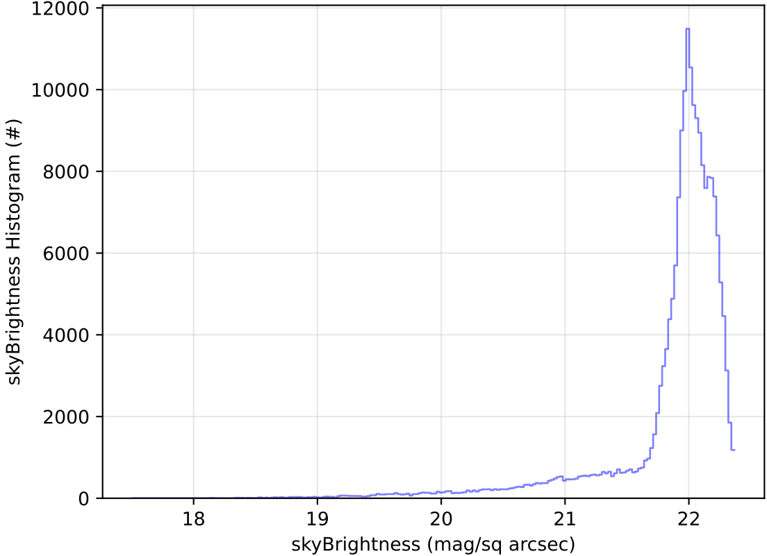
roll_uniform_eh_acc0.2_mjdp0_v3.4_10yrs All sky g band: skyBrightness Histogram
