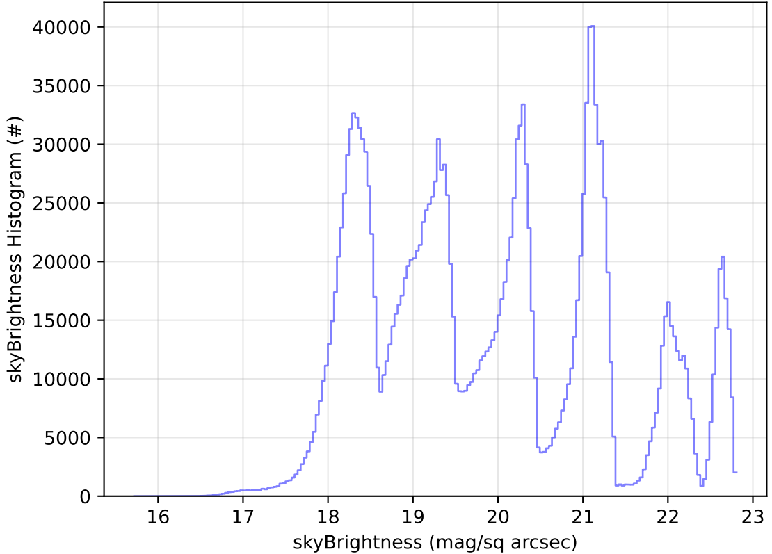
roll_uniform_eh_acc0.2_mjdp0_v3.4_10yrs All sky all bands: skyBrightness Histogram
