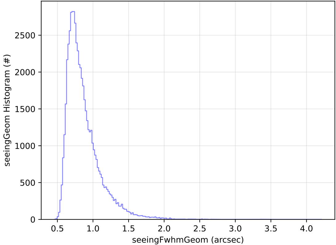
roll_uniform_eh_acc0.2_mjdp0_v3.4_10yrs Yr 1 i band: seeingGeom Histogram
