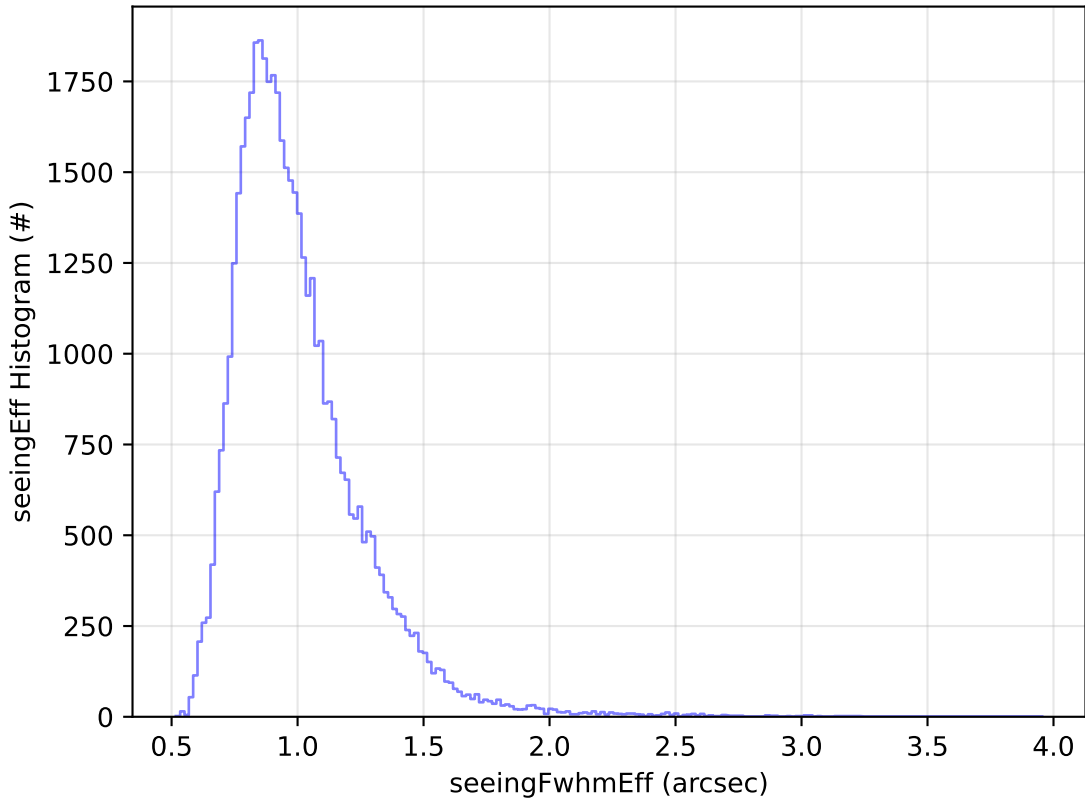
roll_uniform_eh_acc0.2_mjdp0_v3.4_10yrs Yr 1 y band: seeingEff Histogram
