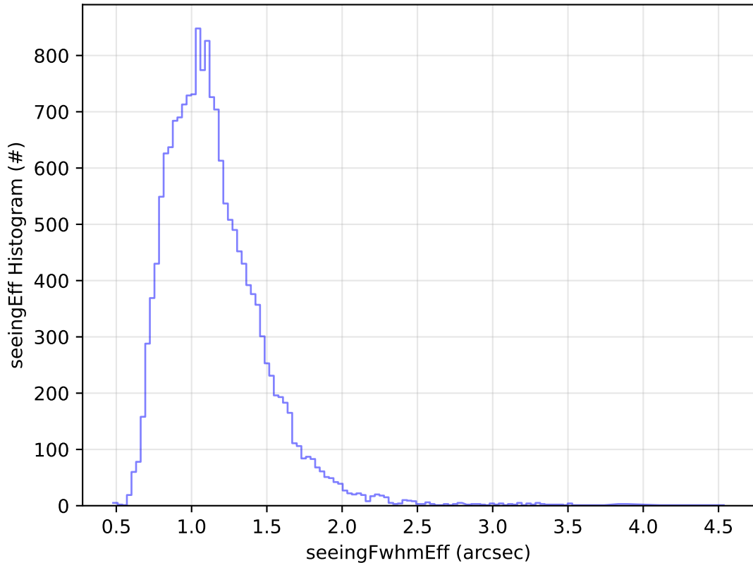
roll_uniform_eh_acc0.2_mjdp0_v3.4_10yrs Yr 1 u band: seeingEff Histogram
