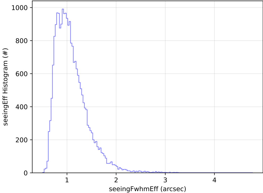
roll_uniform_eh_acc0.2_mjdp0_v3.4_10yrs Yr 1 g band: seeingEff Histogram
