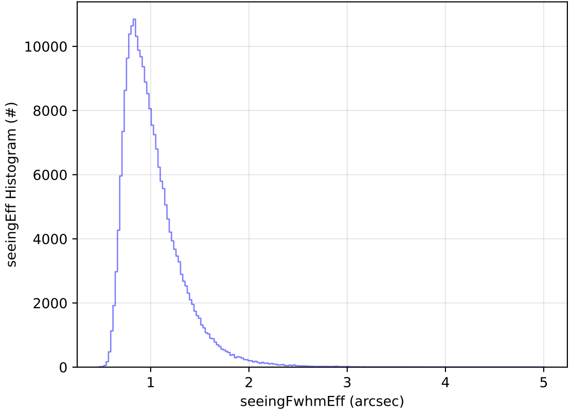
roll_uniform_eh_acc0.2_mjdp0_v3.4_10yrs Yr 1 all bands: seeingEff Histogram
