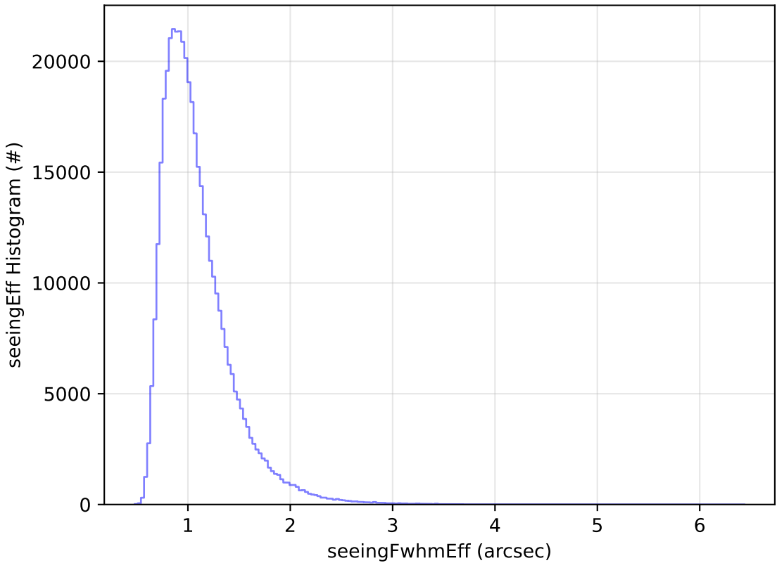
roll_uniform_eh_acc0.2_mjdp0_v3.4_10yrs WFD z band: seeingEff Histogram
