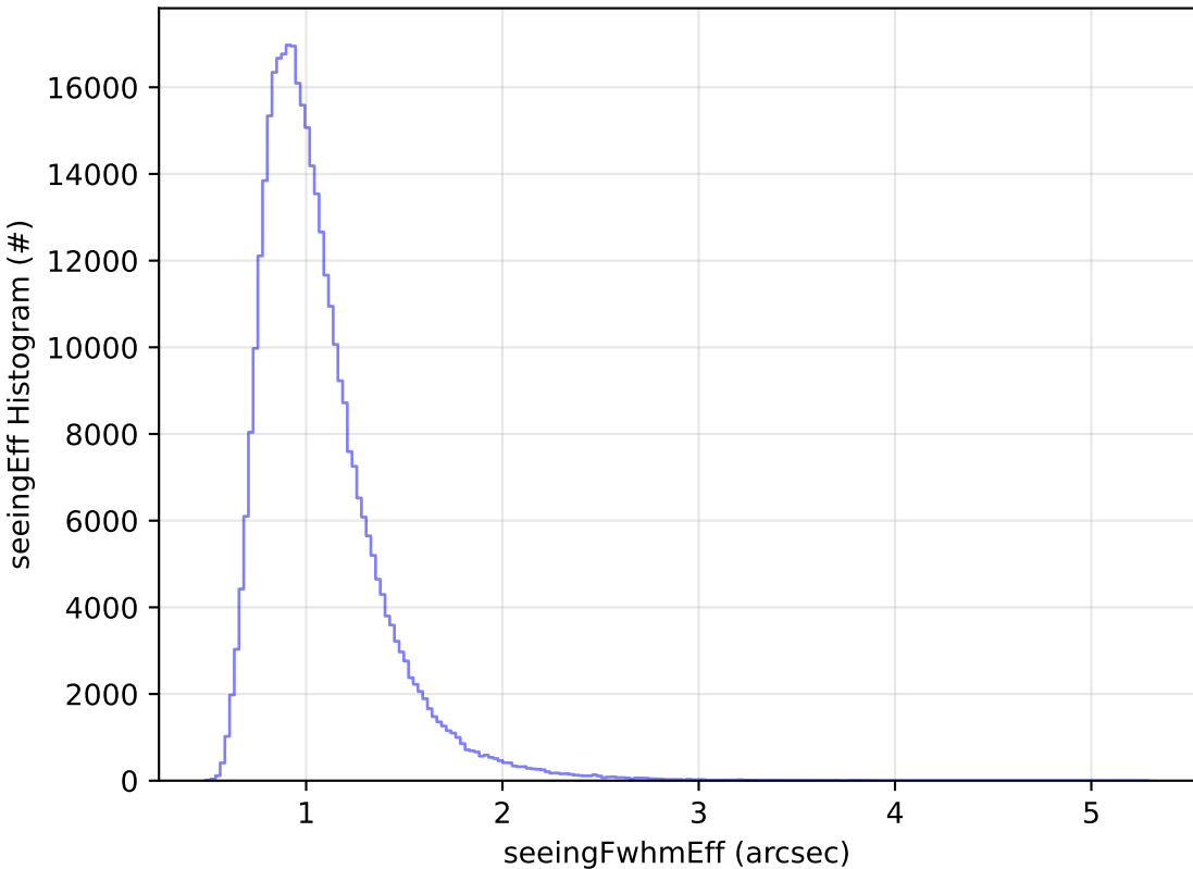
roll_uniform_eh_acc0.2_mjdp0_v3.4_10yrs WFD y band: seeingEff Histogram
