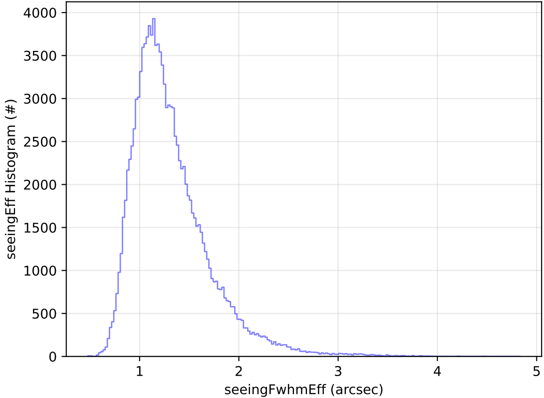
roll_uniform_eh_acc0.2_mjdp0_v3.4_10yrs WFD u band: seeingEff Histogram
