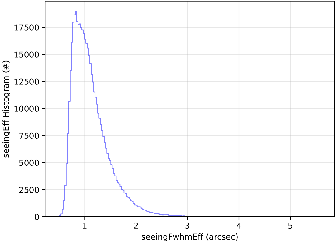
roll_uniform_eh_acc0.2_mjdp0_v3.4_10yrs WFD r band: seeingEff Histogram
