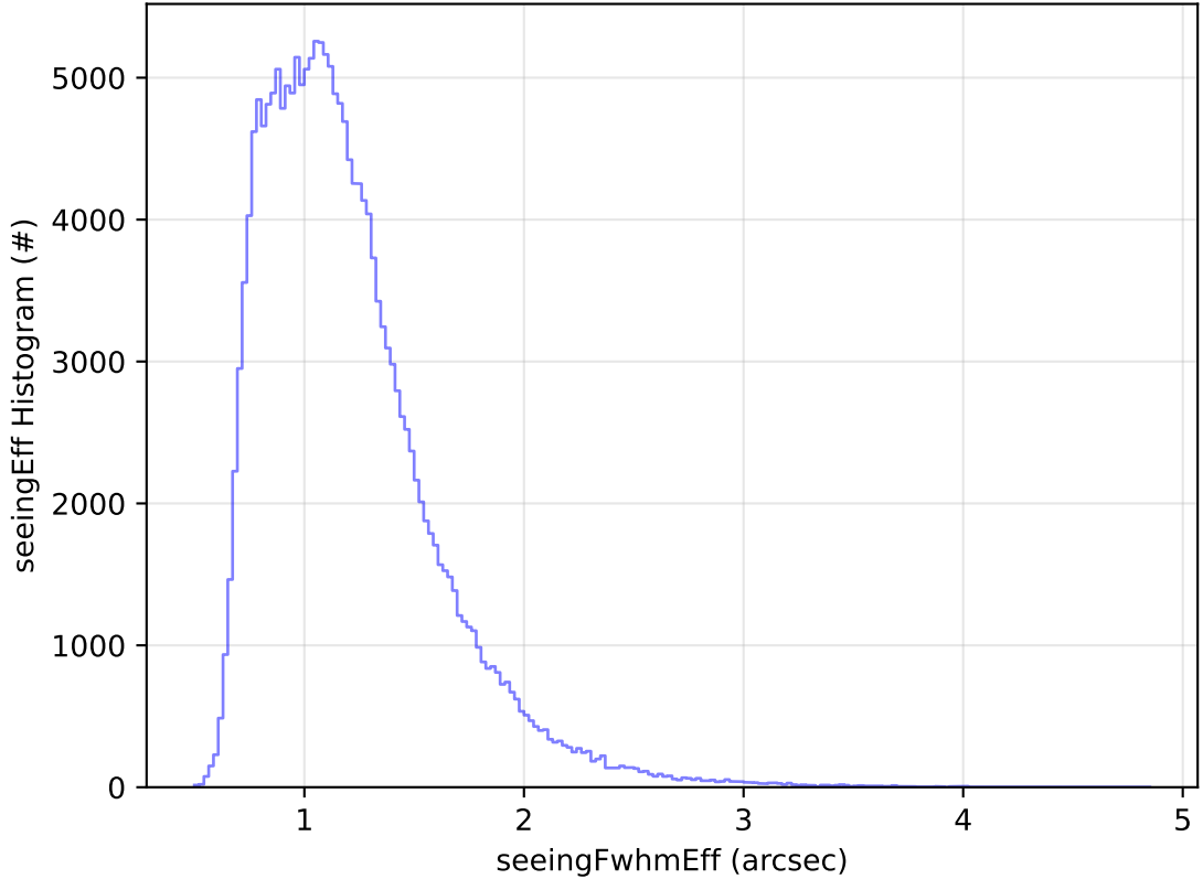
roll_uniform_eh_acc0.2_mjdp0_v3.4_10yrs WFD g band: seeingEff Histogram
