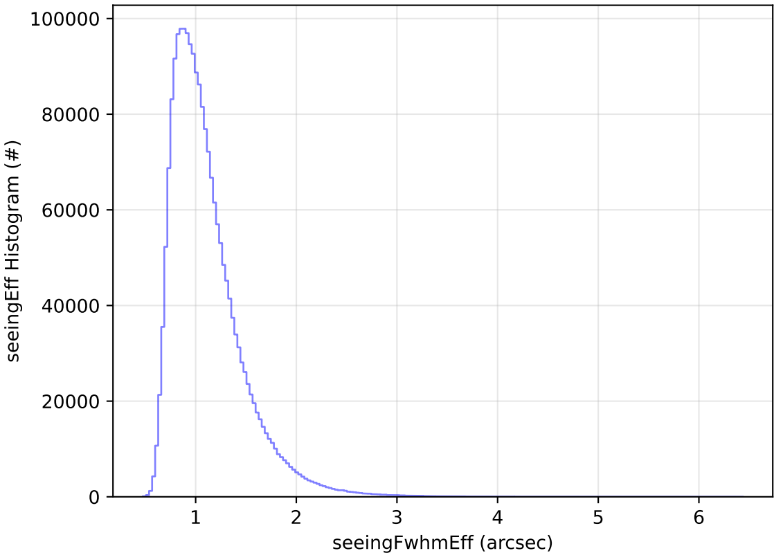
roll_uniform_eh_acc0.2_mjdp0_v3.4_10yrs WFD all bands: seeingEff Histogram
