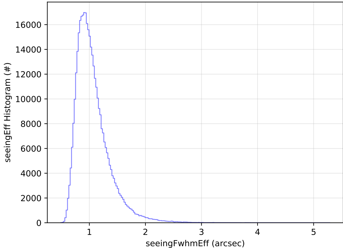
roll_uniform_eh_acc0.2_mjdp0_v3.4_10yrs All sky y band: seeingEff Histogram
