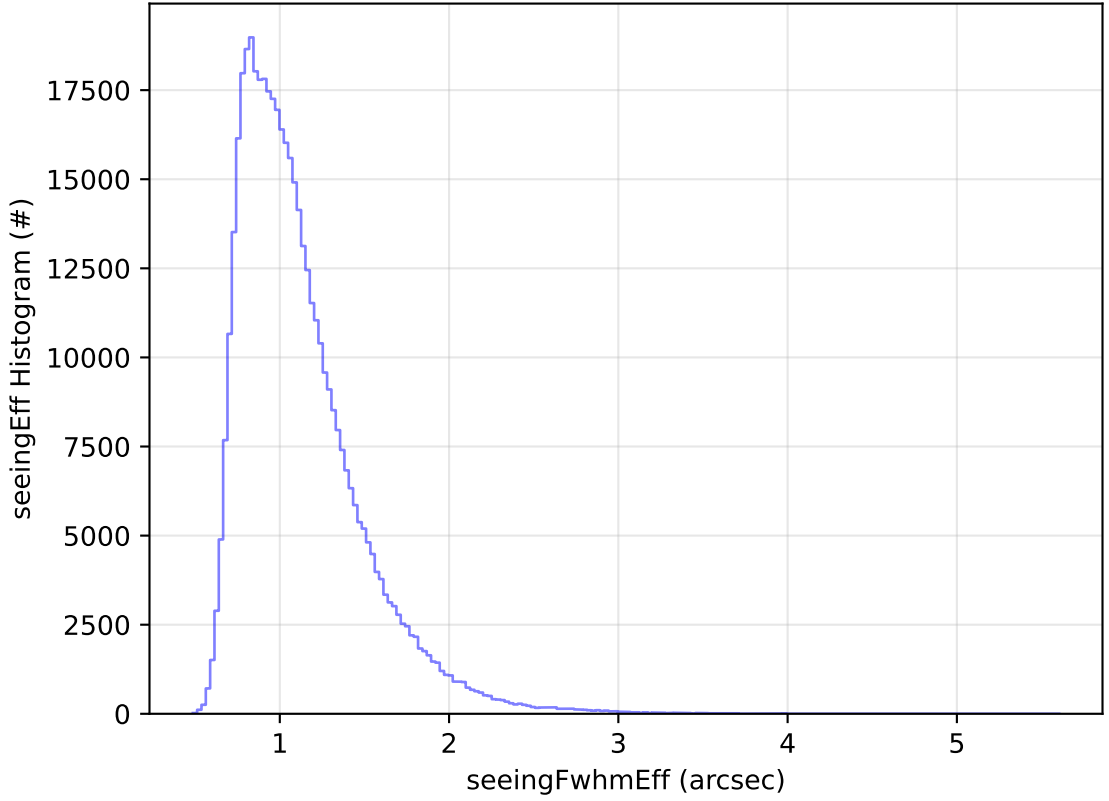
roll_uniform_eh_acc0.2_mjdp0_v3.4_10yrs All sky r band: seeingEff Histogram
