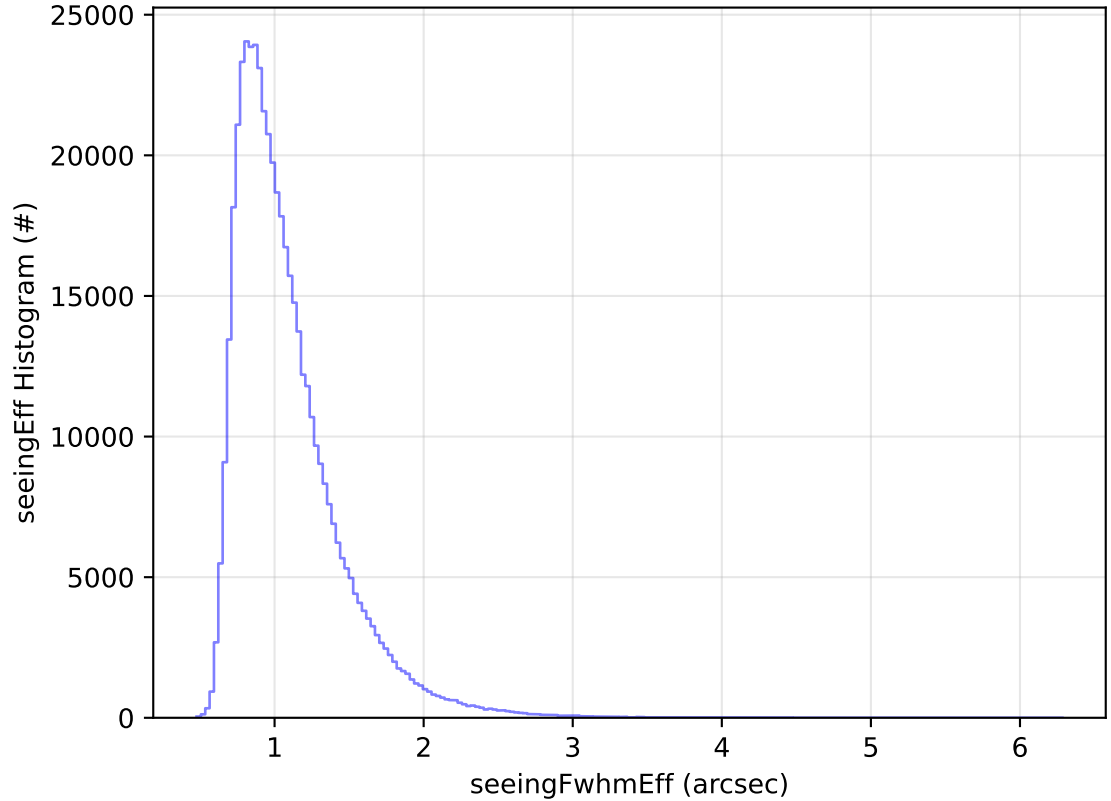
roll_uniform_eh_acc0.2_mjdp0_v3.4_10yrs All sky i band: seeingEff Histogram
