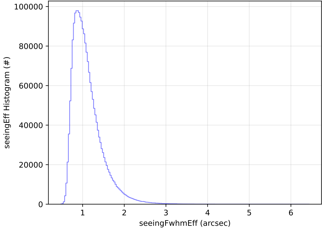
roll_uniform_eh_acc0.2_mjdp0_v3.4_10yrs All sky all bands: seeingEff Histogram
