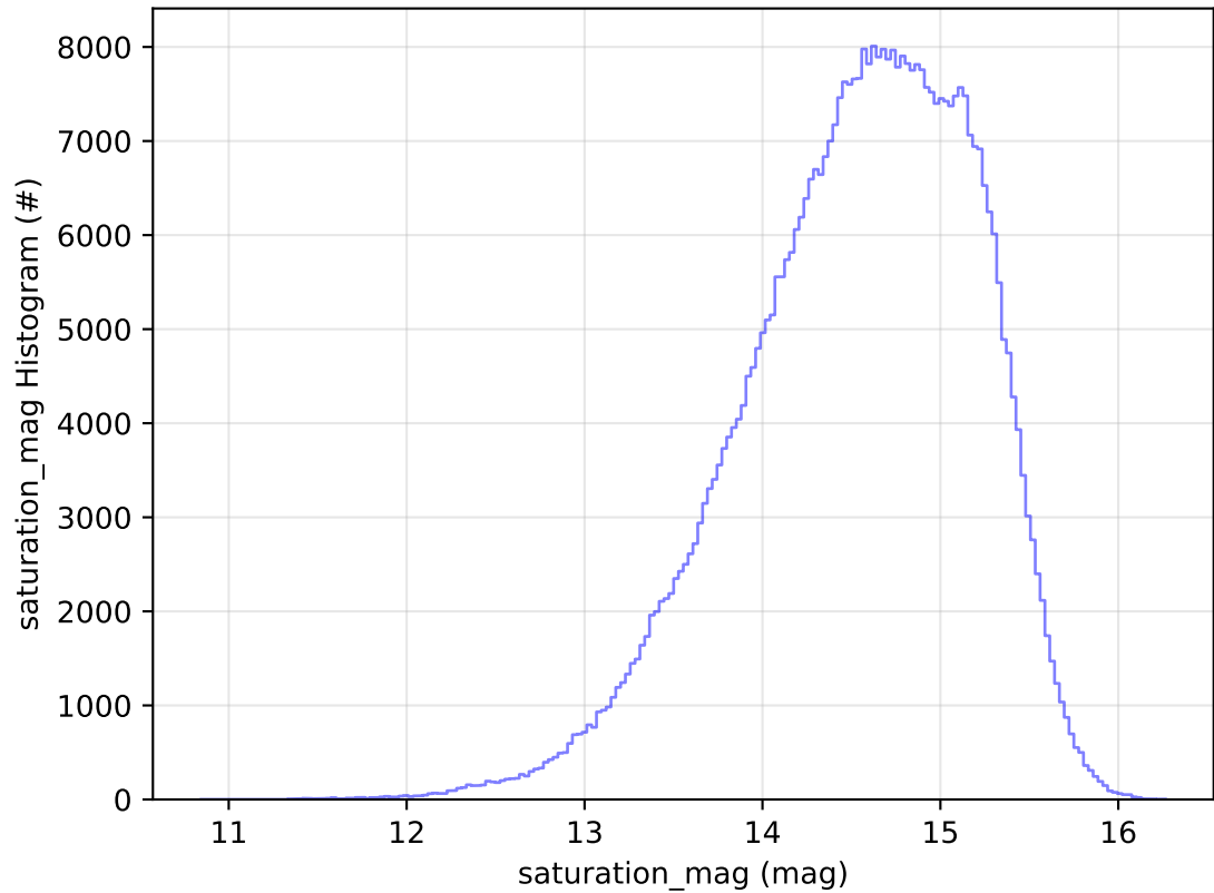
roll_uniform_eh_acc0.2_mjdp0_v3.4_10yrs WFD r band: saturation_mag Histogram
