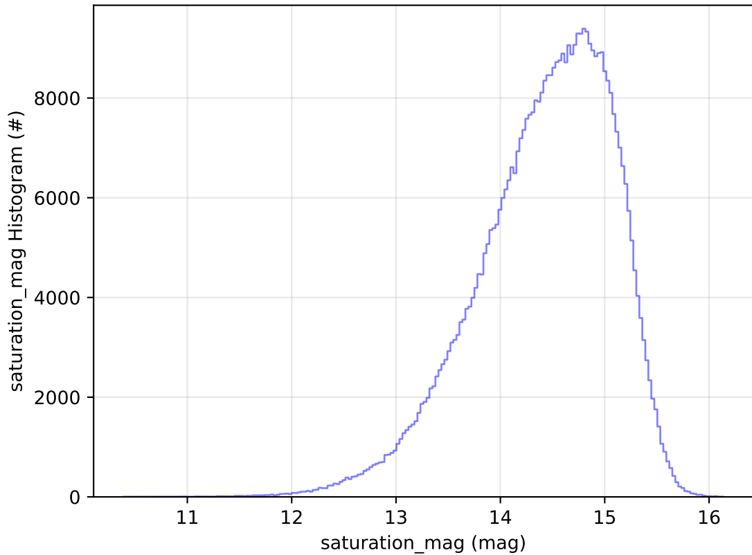
roll_uniform_eh_acc0.2_mjdp0_v3.4_10yrs WFD i band: saturation_mag Histogram
