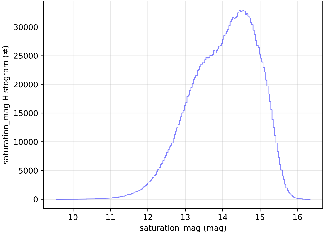
roll_uniform_eh_acc0.2_mjdp0_v3.4_10yrs WFD all bands: saturation_mag Histogram
