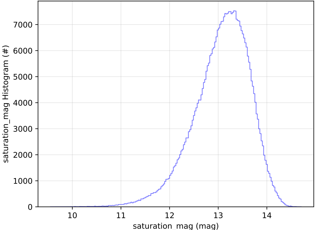
roll_uniform_eh_acc0.2_mjdp0_v3.4_10yrs All sky y band: saturation_mag Histogram
