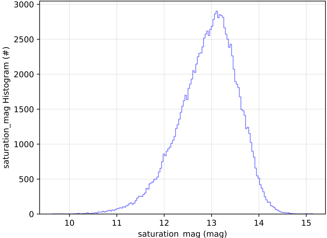
roll_uniform_eh_acc0.2_mjdp0_v3.4_10yrs All sky u band: saturation_mag Histogram
