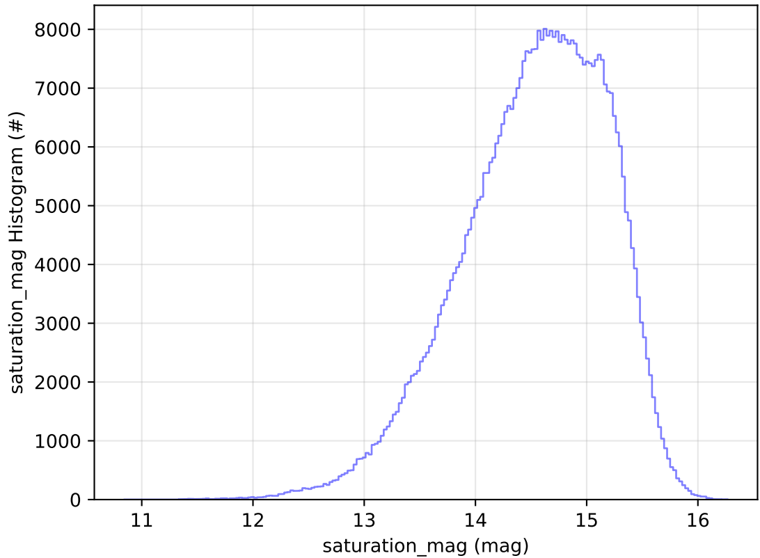
roll_uniform_eh_acc0.2_mjdp0_v3.4_10yrs All sky r band: saturation_mag Histogram
