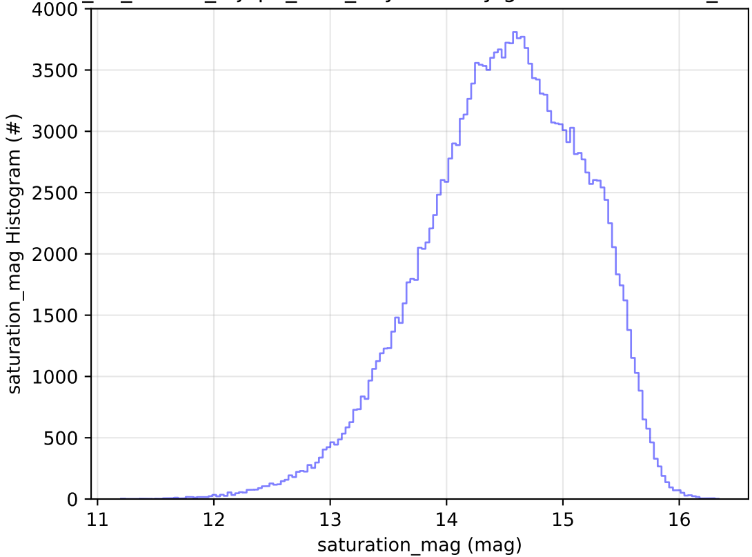
roll_uniform_eh_acc0.2_mjdp0_v3.4_10yrs All sky g band: saturation_mag Histogram
