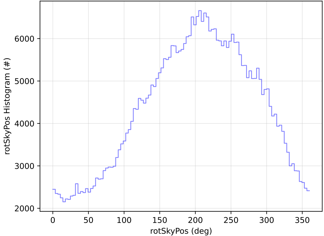
roll_uniform_eh_acc0.2_mjdp0_v3.4_10yrs WFD z band: rotSkyPos Histogram
