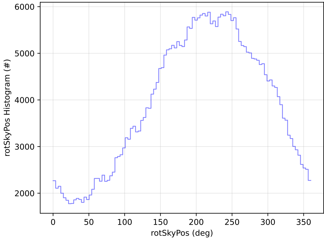
roll_uniform_eh_acc0.2_mjdp0_v3.4_10yrs WFD y band: rotSkyPos Histogram
