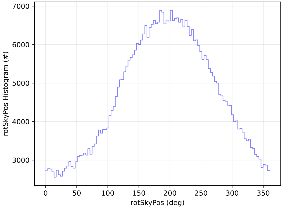
roll_uniform_eh_acc0.2_mjdp0_v3.4_10yrs WFD r band: rotSkyPos Histogram
