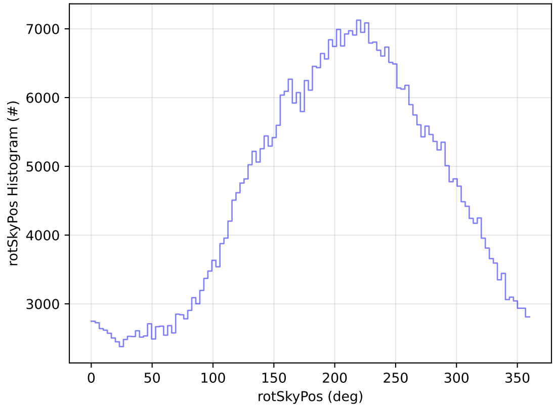
roll_uniform_eh_acc0.2_mjdp0_v3.4_10yrs WFD i band: rotSkyPos Histogram
