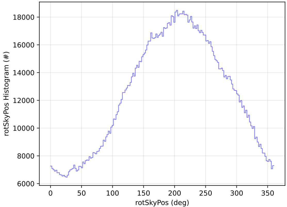
roll_uniform_eh_acc0.2_mjdp0_v3.4_10yrs WFD all bands: rotSkyPos Histogram
