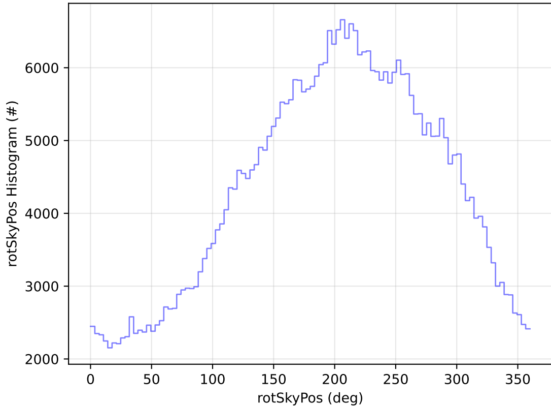
roll_uniform_eh_acc0.2_mjdp0_v3.4_10yrs All sky z band: rotSkyPos Histogram
