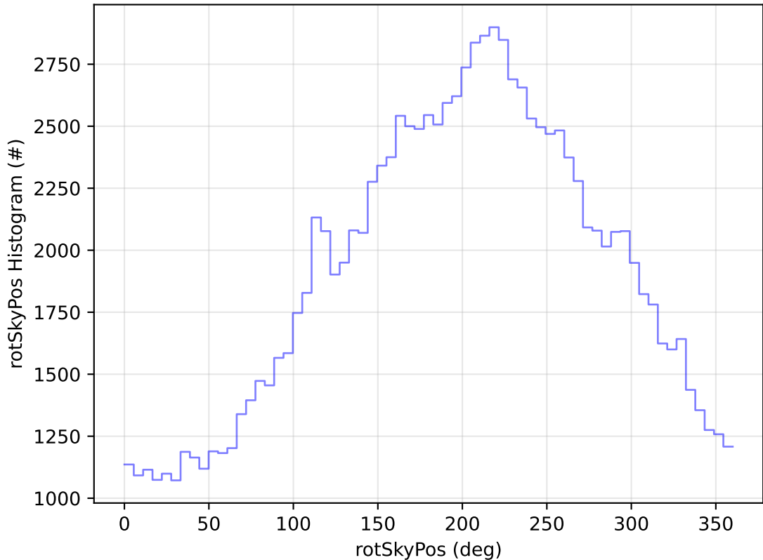
roll_uniform_eh_acc0.2_mjdp0_v3.4_10yrs All sky u band: rotSkyPos Histogram
