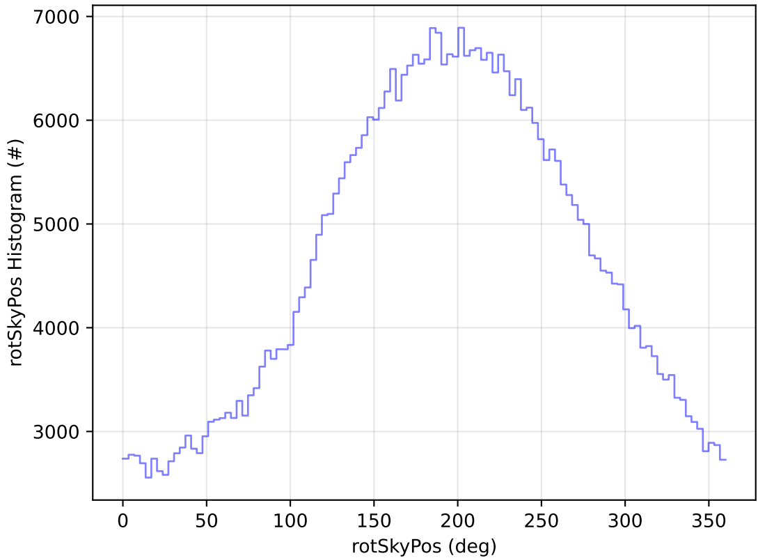
roll_uniform_eh_acc0.2_mjdp0_v3.4_10yrs All sky r band: rotSkyPos Histogram
