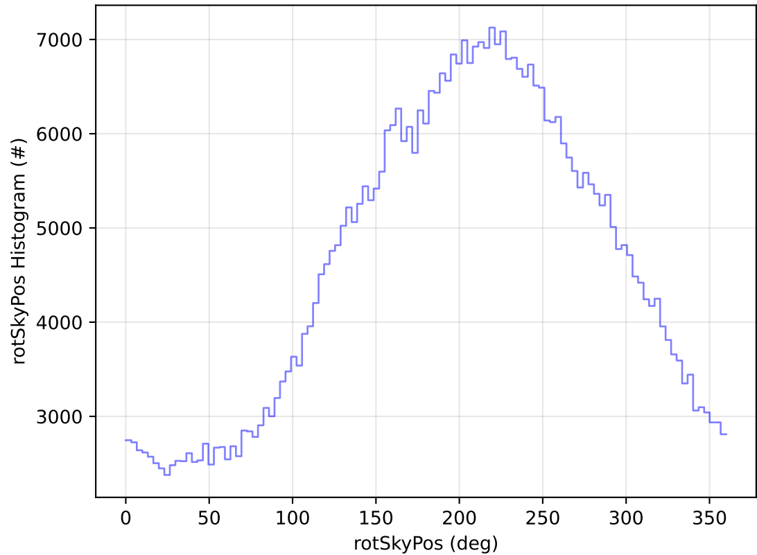
roll_uniform_eh_acc0.2_mjdp0_v3.4_10yrs All sky i band: rotSkyPos Histogram
