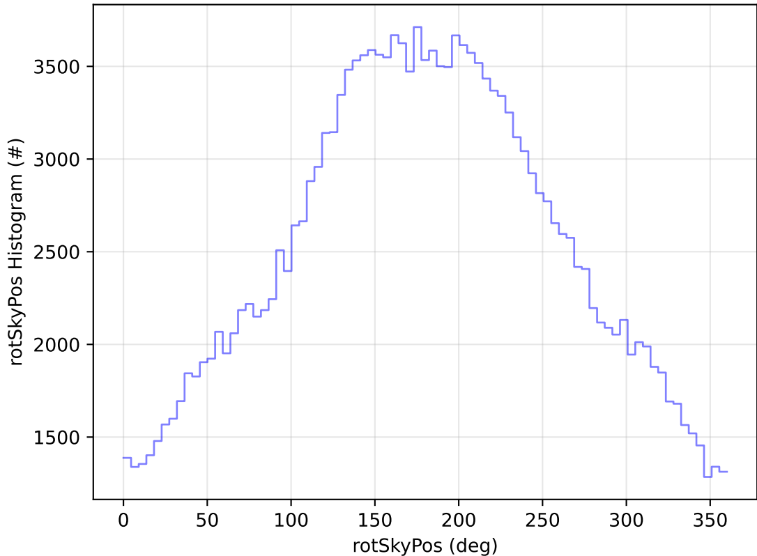
roll_uniform_eh_acc0.2_mjdp0_v3.4_10yrs All sky g band: rotSkyPos Histogram
