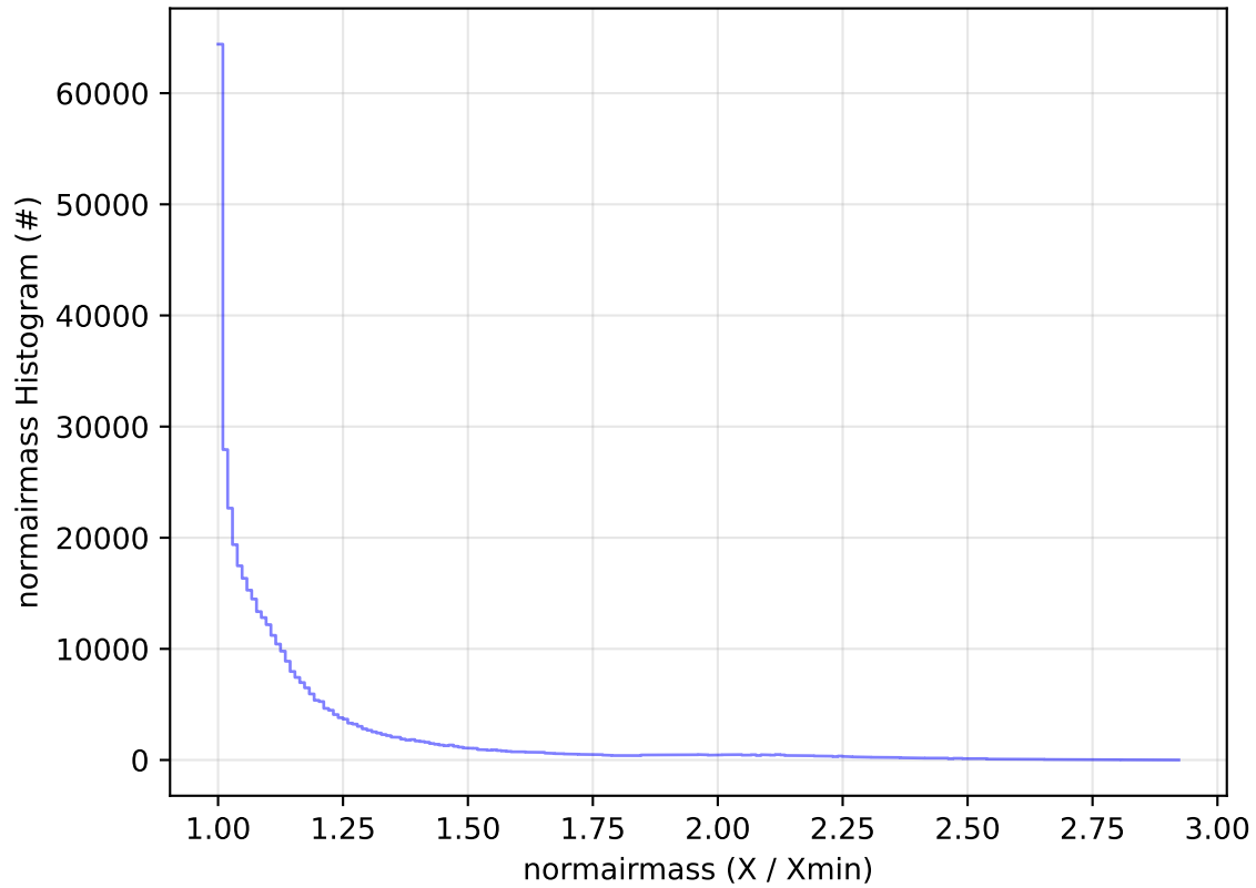
roll_uniform_eh_acc0.2_mjdp0_v3.4_10yrs WFD z band: normairmass Histogram
