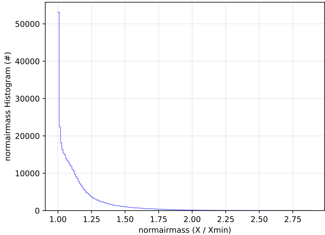
roll_uniform_eh_acc0.2_mjdp0_v3.4_10yrs WFD y band: normairmass Histogram
