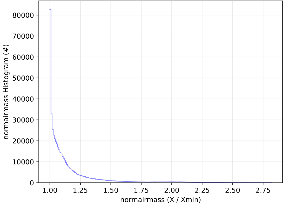
roll_uniform_eh_acc0.2_mjdp0_v3.4_10yrs WFD r band: normairmass Histogram
