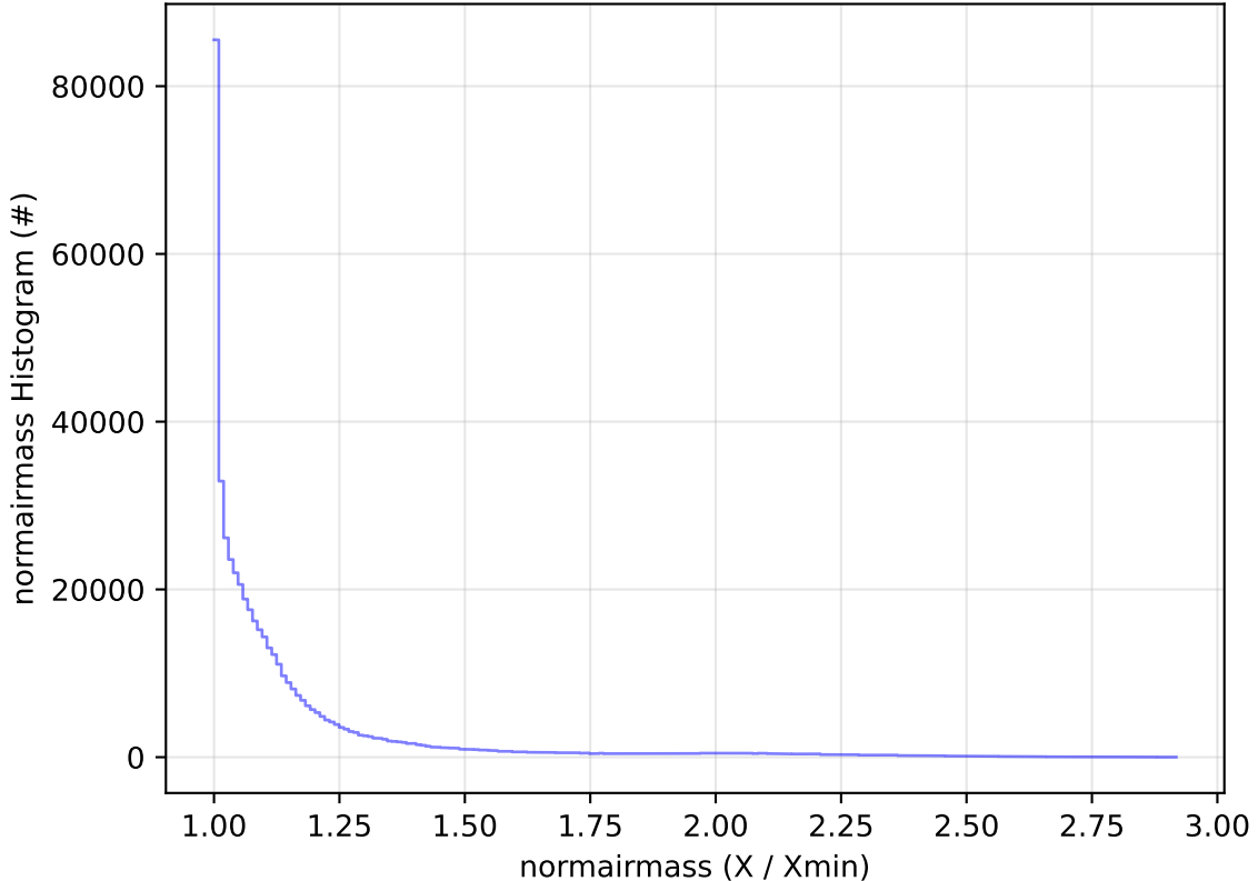
roll_uniform_eh_acc0.2_mjdp0_v3.4_10yrs WFD i band: normairmass Histogram
