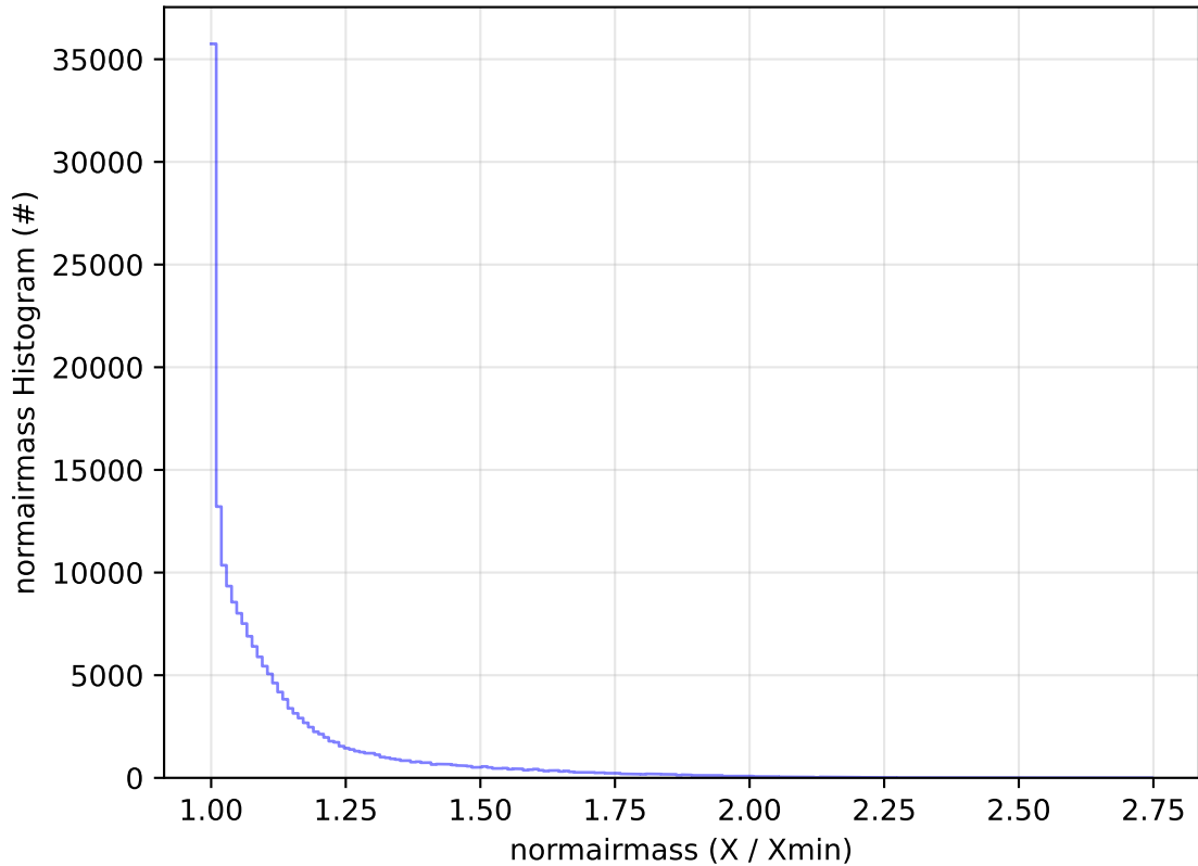
roll_uniform_eh_acc0.2_mjdp0_v3.4_10yrs WFD g band: normairmass Histogram
