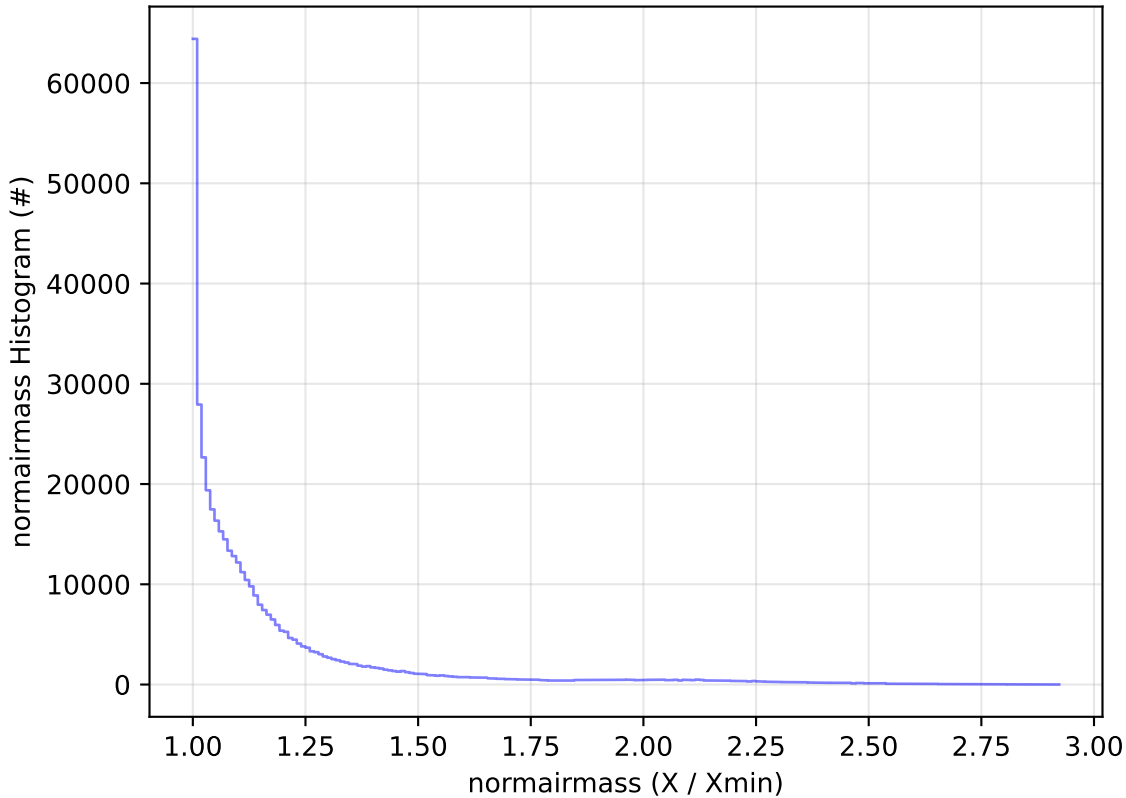
roll_uniform_eh_acc0.2_mjdp0_v3.4_10yrs All sky z band: normairmass Histogram
