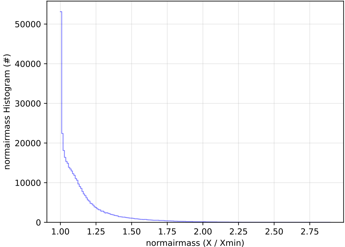
roll_uniform_eh_acc0.2_mjdp0_v3.4_10yrs All sky y band: normairmass Histogram
