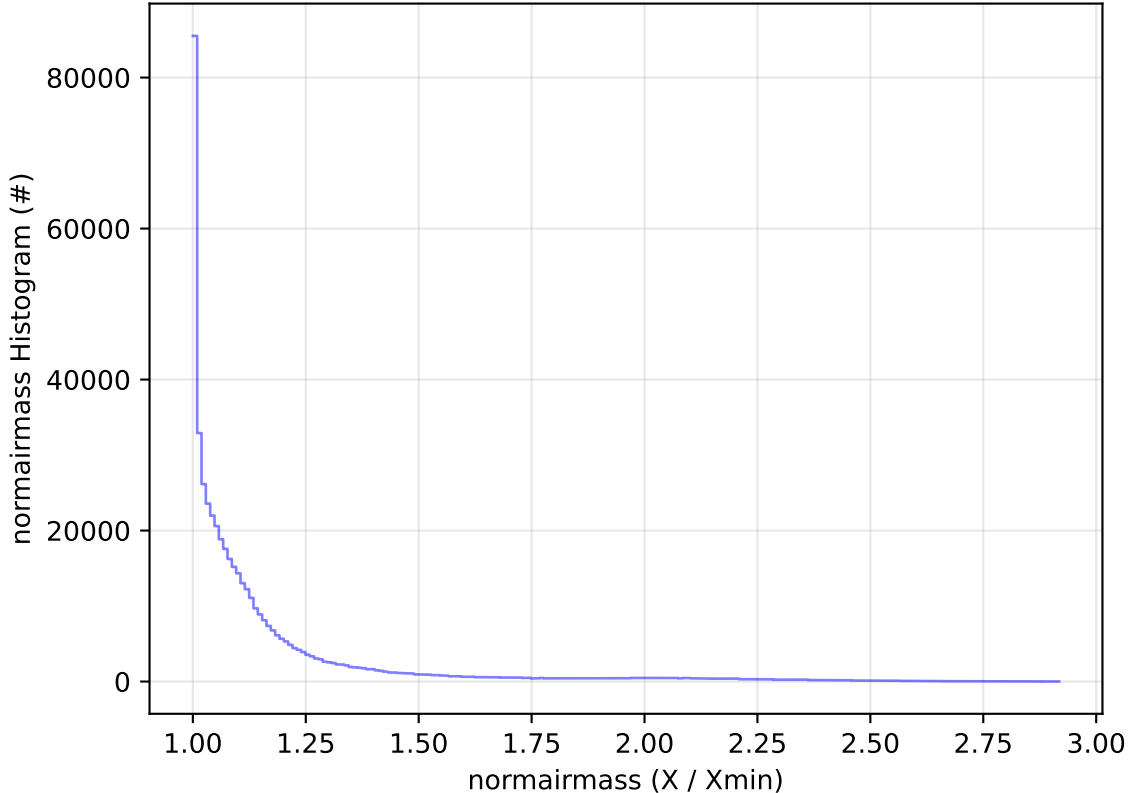
roll_uniform_eh_acc0.2_mjdp0_v3.4_10yrs All sky i band: normairmass Histogram
