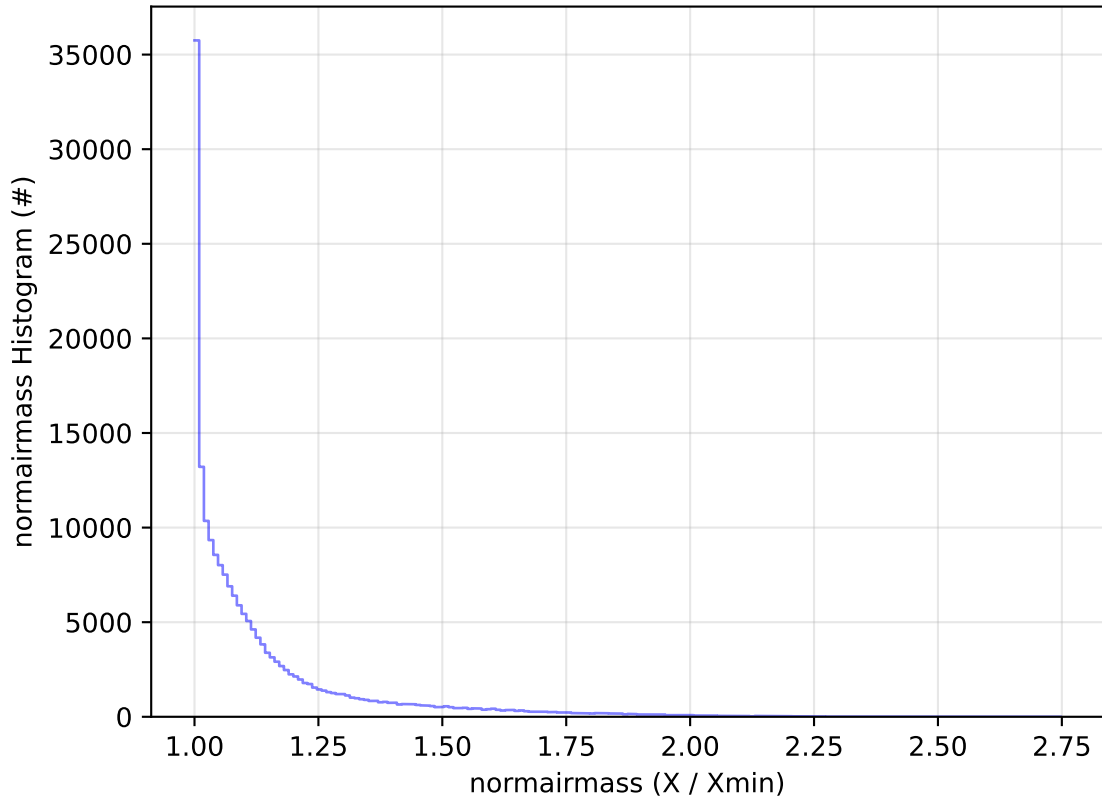
roll_uniform_eh_acc0.2_mjdp0_v3.4_10yrs All sky g band: normairmass Histogram
