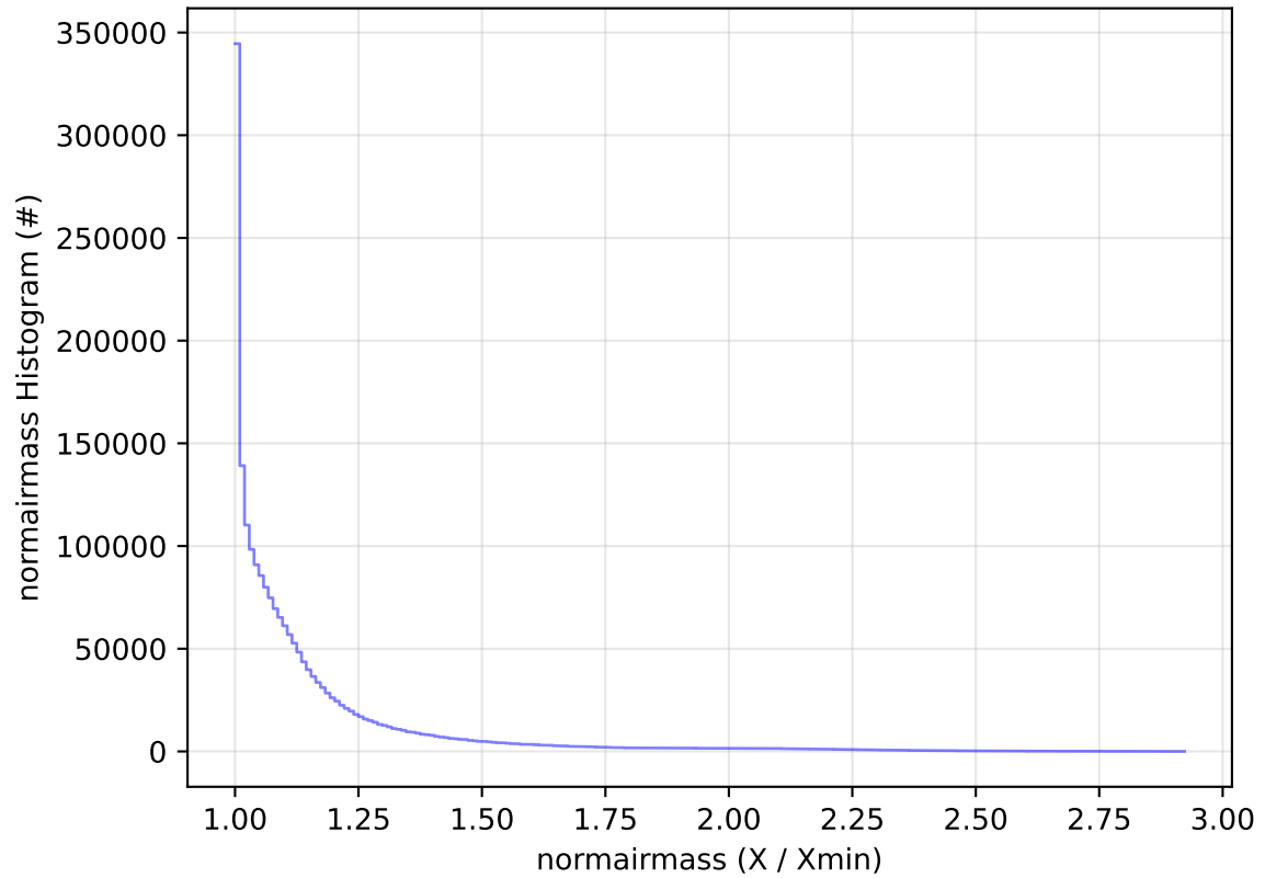
roll_uniform_eh_acc0.2_mjdp0_v3.4_10yrs All sky all bands: normairmass Histogram
