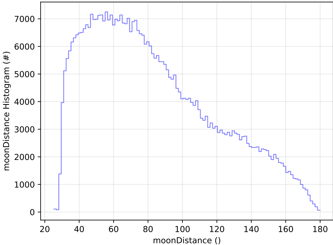
roll_uniform_eh_acc0.2_mjdp0_v3.4_10yrs WFD z band: moonDistance Histogram
