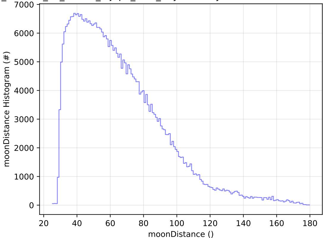
roll_uniform_eh_acc0.2_mjdp0_v3.4_10yrs WFD y band: moonDistance Histogram
