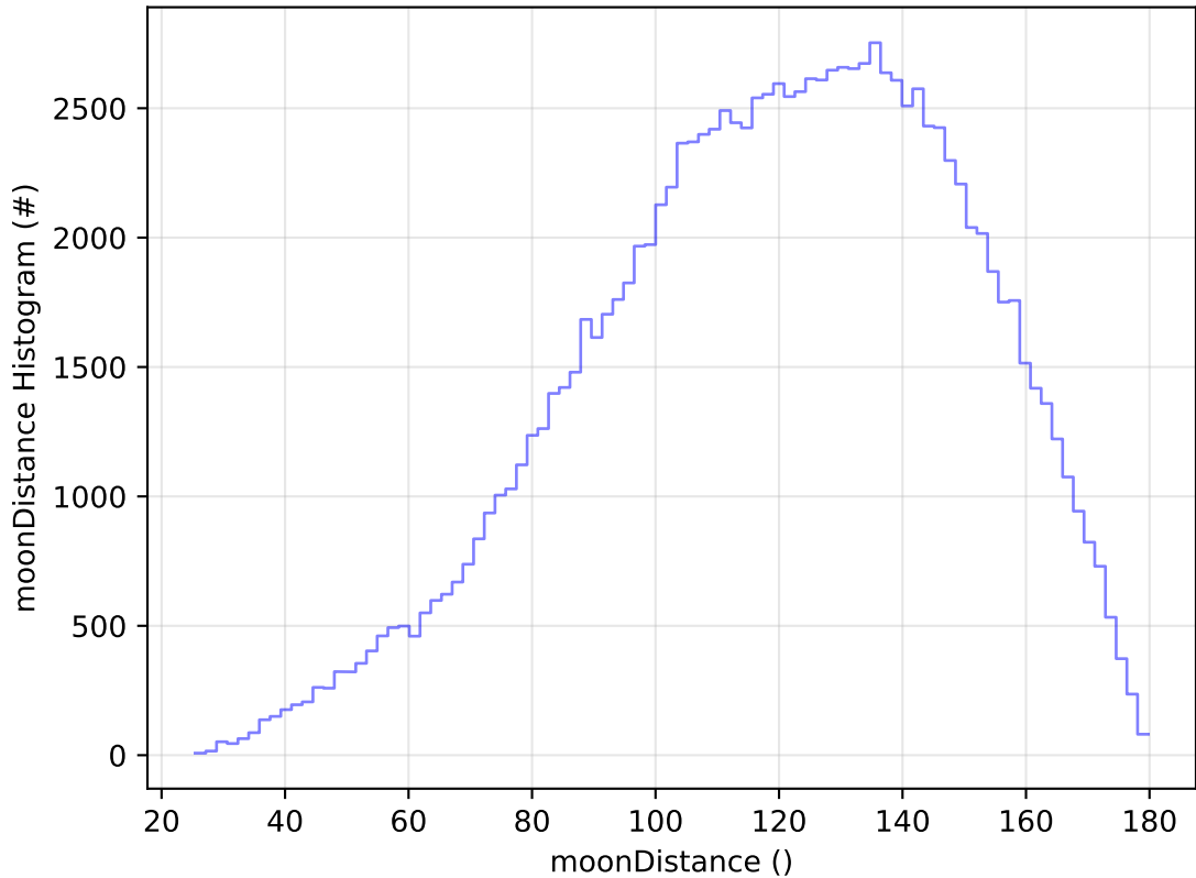
roll_uniform_eh_acc0.2_mjdp0_v3.4_10yrs WFD u band: moonDistance Histogram
