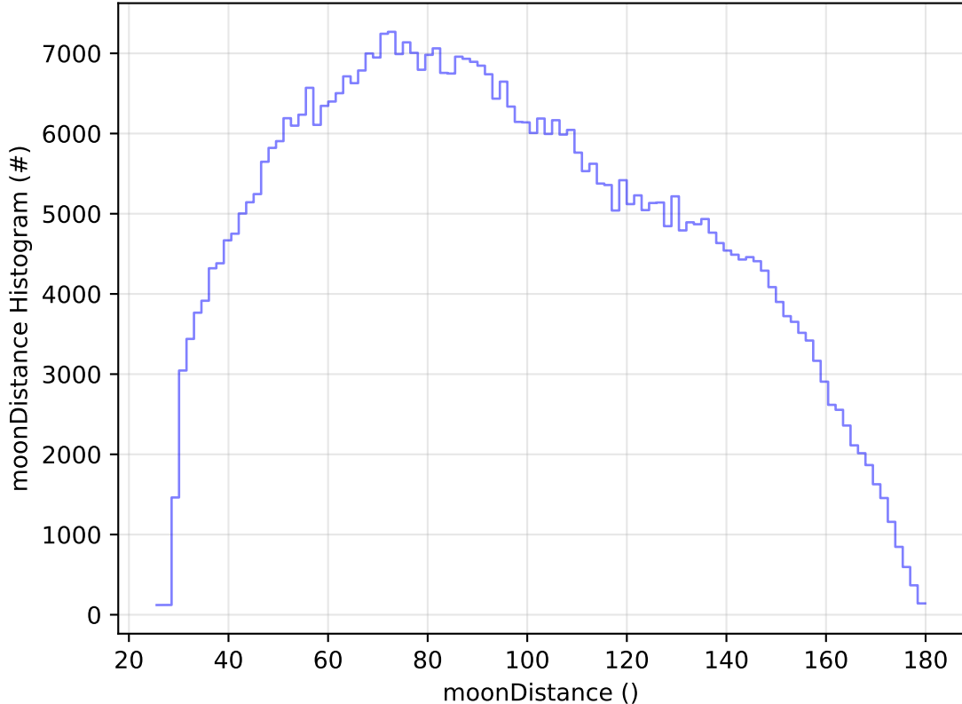
roll_uniform_eh_acc0.2_mjdp0_v3.4_10yrs WFD i band: moonDistance Histogram
