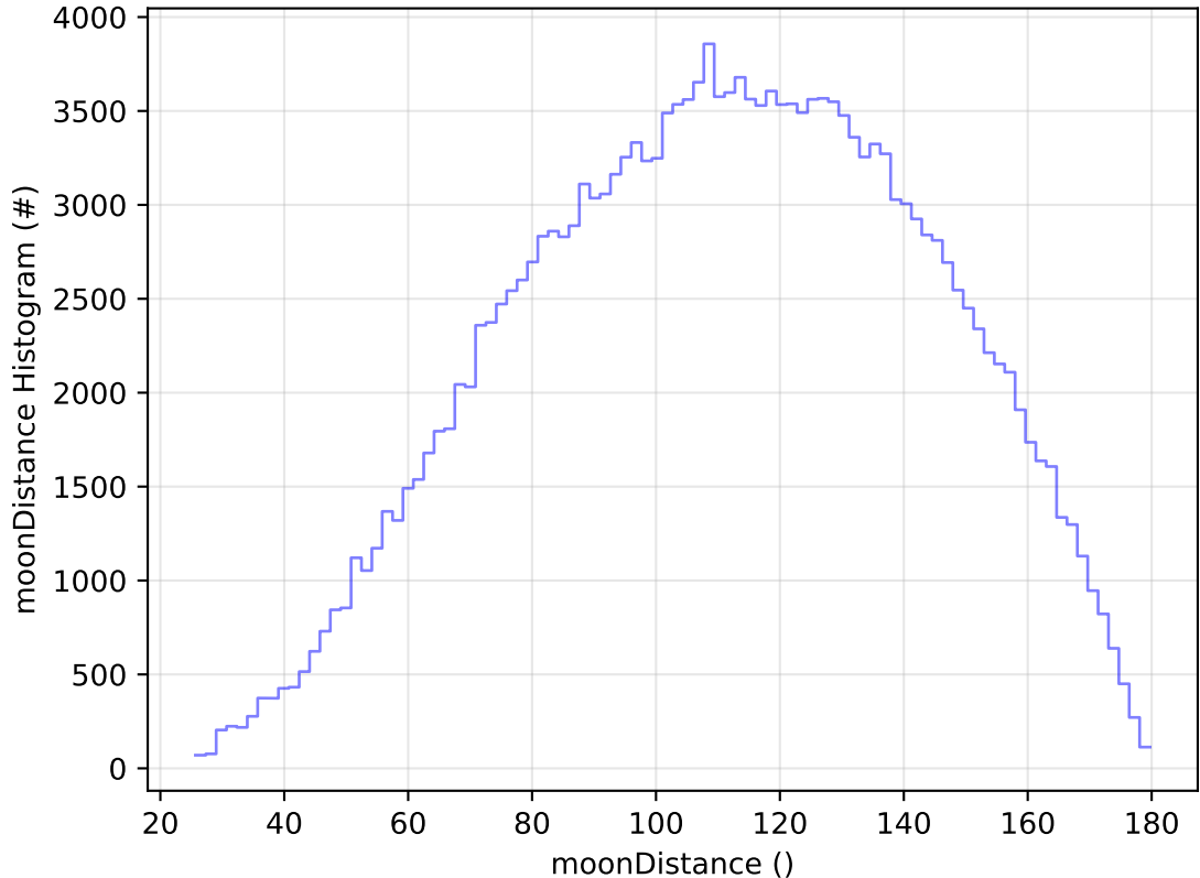
roll_uniform_eh_acc0.2_mjdp0_v3.4_10yrs WFD g band: moonDistance Histogram
